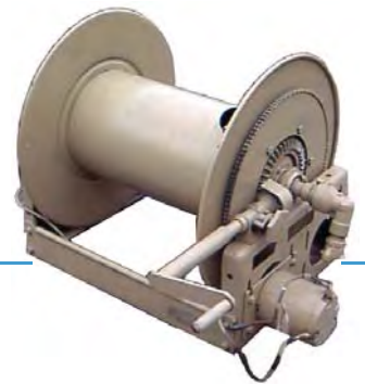
Hose reel 12V electric and hand crank for 225' of 3/4" I.D. air hose
